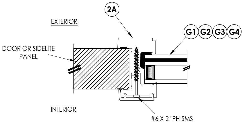
SECTION THROUGH LITE FRAME
